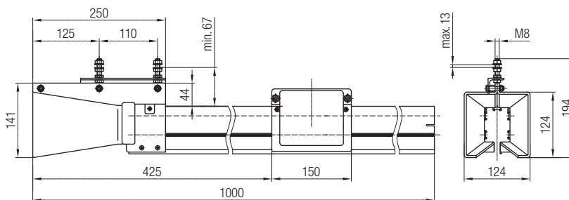
4/5 poles - type "left" for CS (continuous strip)
