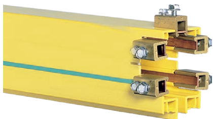
System JT (joint clamping)
